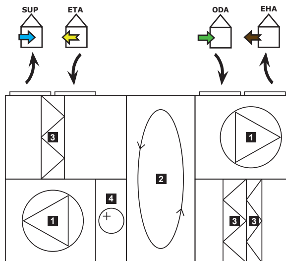
Operational diagram left version upper connections
