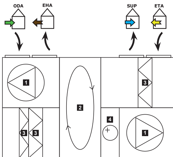
Operational diagram right version upper connections
